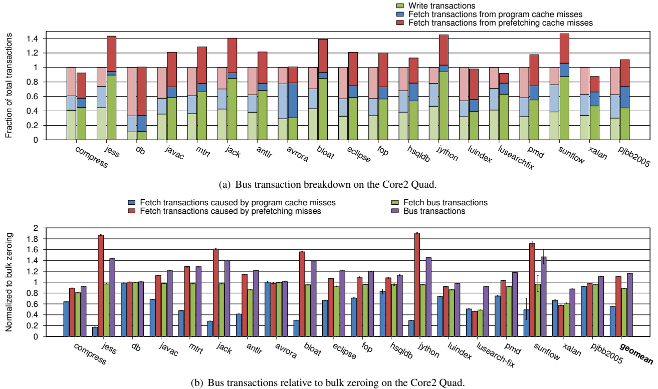
Figure 12. Memory bus utilization: Non-temporal bulk zeroing/bulk zeroing
