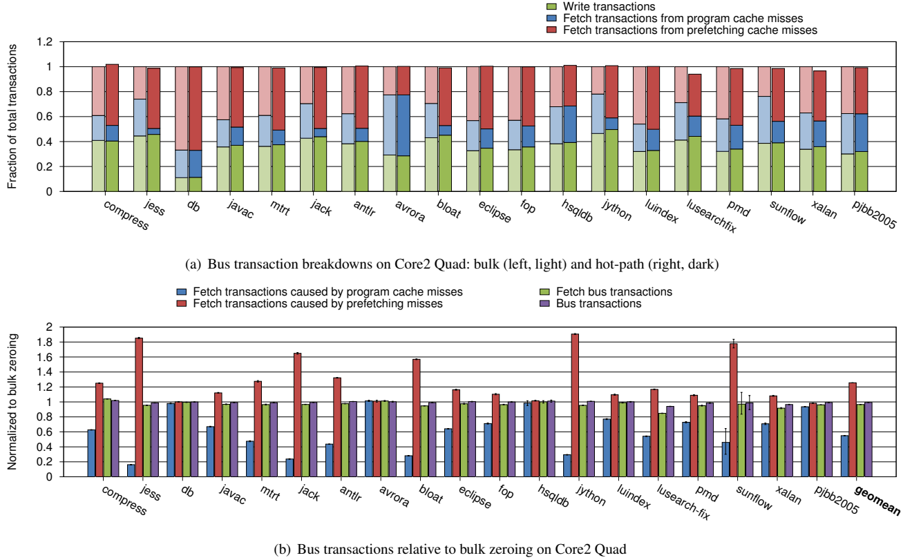
Figure 7. Memory bus utilization: hot-path/bulk zeroing
