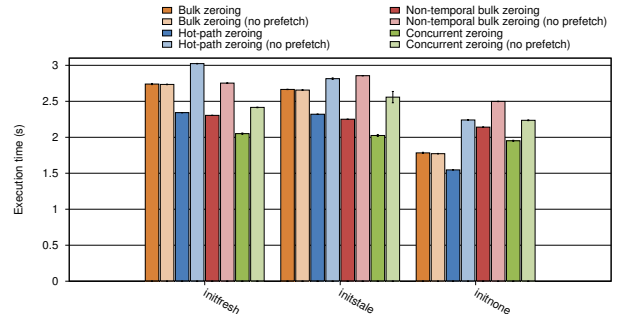
Figure 9. Execution time of microbenchmarks on Core2 Quad with and without hardware prefetch enabled
