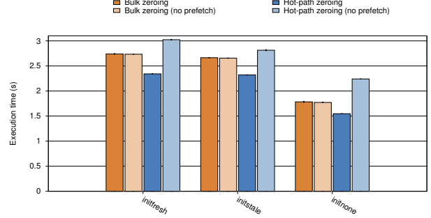
Figure 5. Execution time of microbenchmarks on Core2 Quad with and without hardware prefetch enabled
